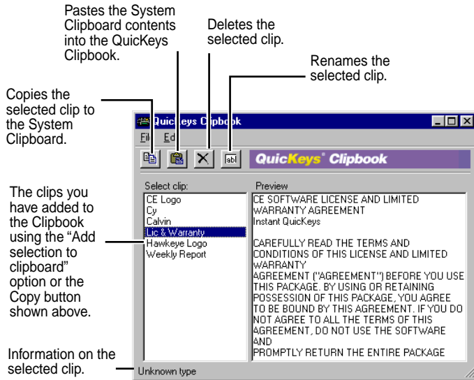
FIGURE 113: The Clipbook Editor
