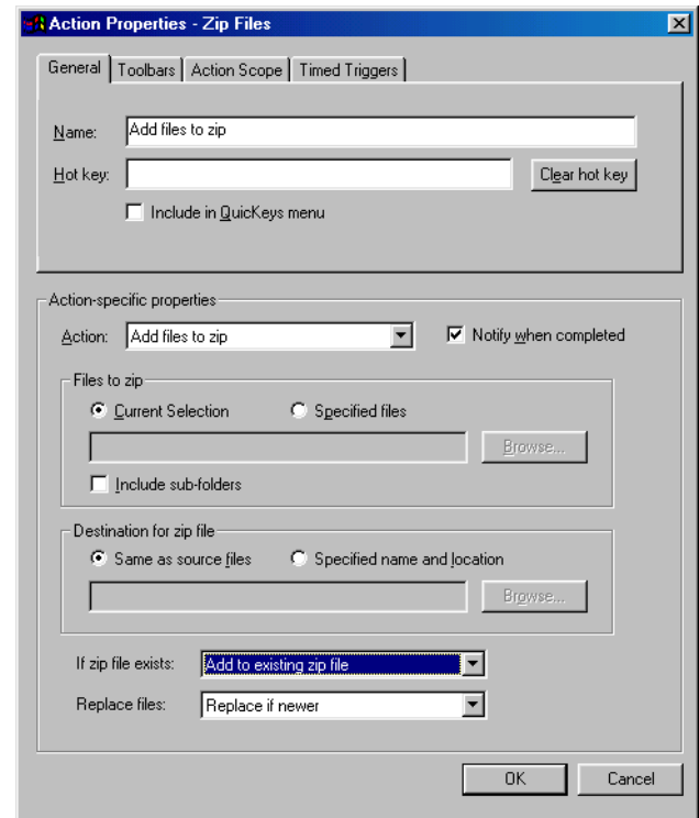
FIGURE 104: The Zip Files Action Properties dialog appears when you select Zip Files from the Create menu, or when you double-click an existing Zip Files Action in the My Actions tab.
