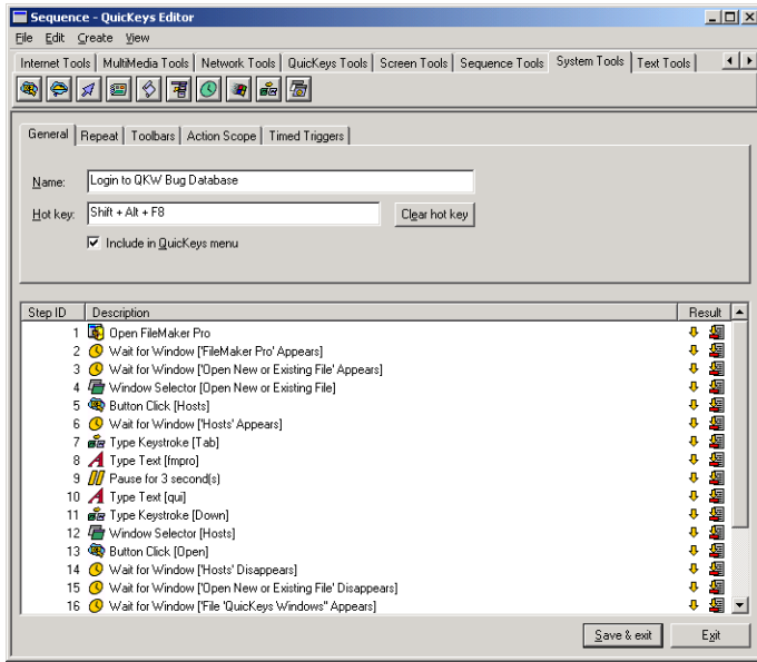
FIGURE 161: A Sequence Scope that automates logging into a database program.
