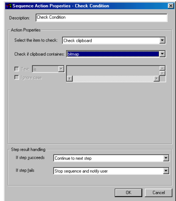
FIGURE 177: The Check clipboard Action Properties
