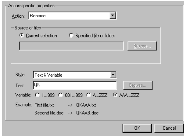
FIGURE 92: The Text & Variable option
