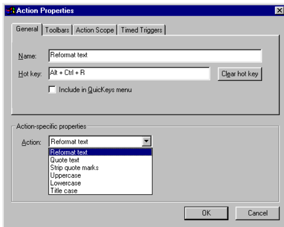
FIGURE 65: The Advanced Text Tools Action Properties dialog appears when you select the Advanced Text Tools Action from the Create menu, or when you double-click an existing Advanced Text Tools Action in the My Actions tab.
