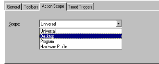
FIGURE 17: The Action Properties Action Scope tab If you have already scoped an Action to an application, that application appears at the top of the scope list.
