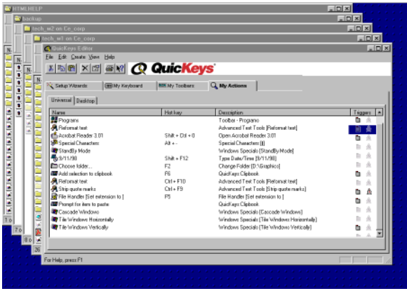
FIGURE 132: Cascading windows
