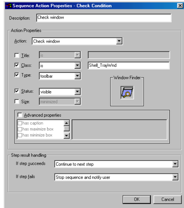
FIGURE 175: The Check window Action Properties
