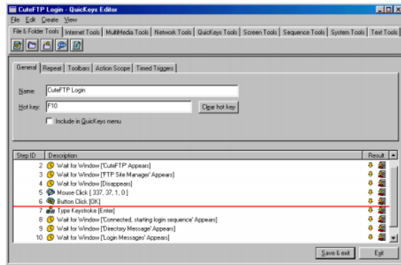
FIGURE 163: The Sequence Editor
