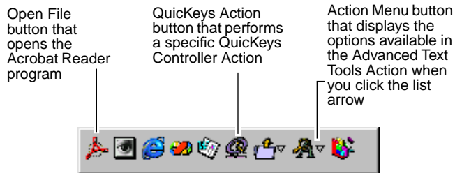
FIGURE 47: In this example, you can see what each type of toolbar button looks like. An Open File button uses the icon of the file it opens, a QuickKeys Action button uses the icon of the QuickKeys Action it opens, and an Action Menu button uses the icon of the QuickKeys Action it opens along with a drop-down arrow.
