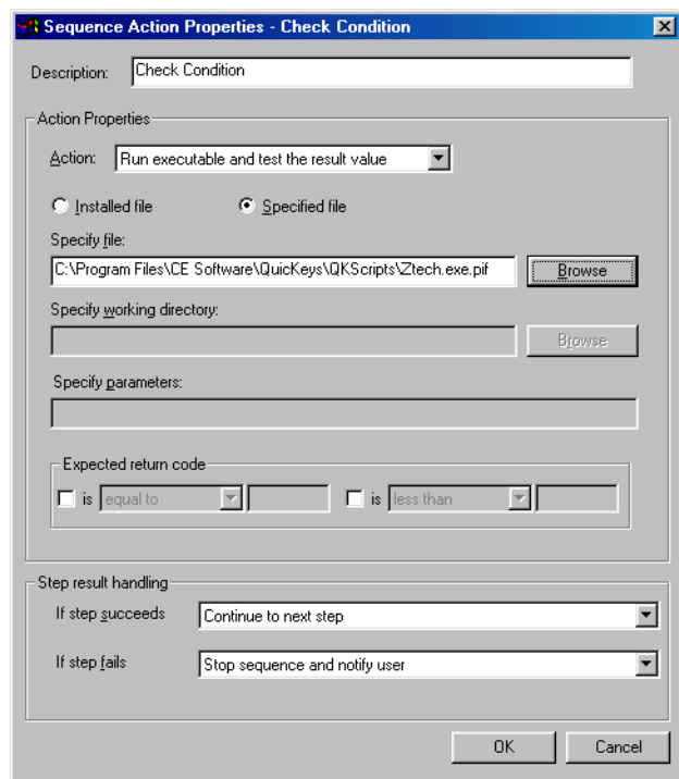
FIGURE 180: Run an executable from an installed file or from a specified file.
